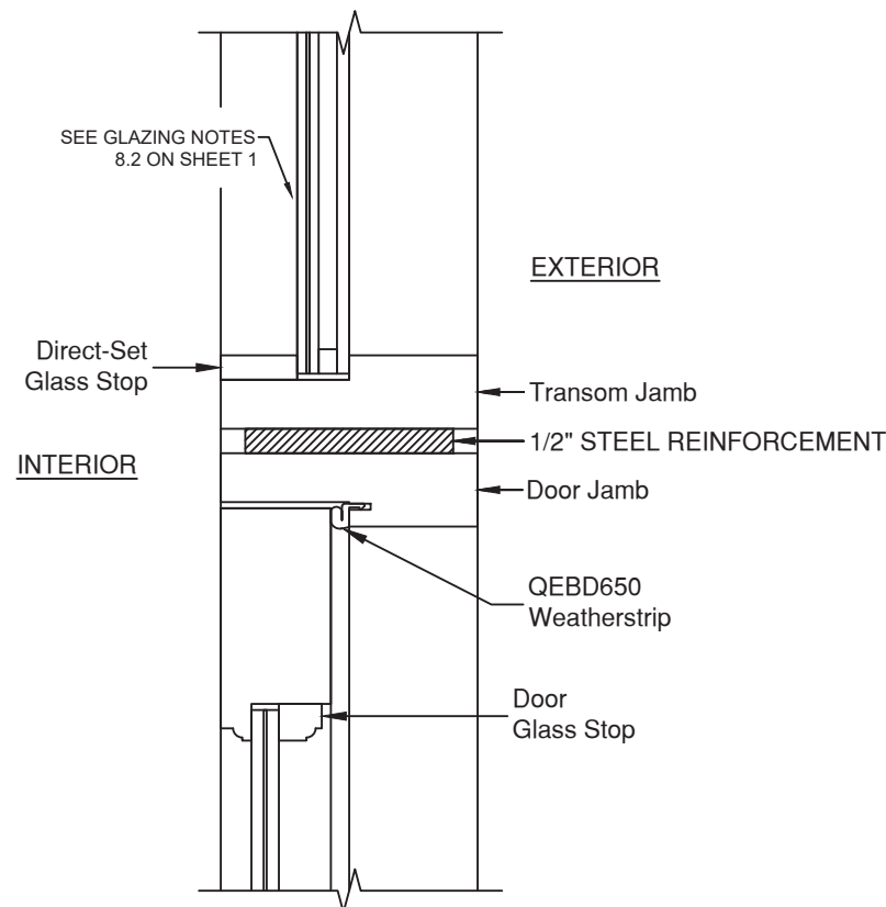
O 10 HORIZONTAL MULL W/ DOOR AND DIRECT SET TRANSOM HORIZONTAL DETAIL
